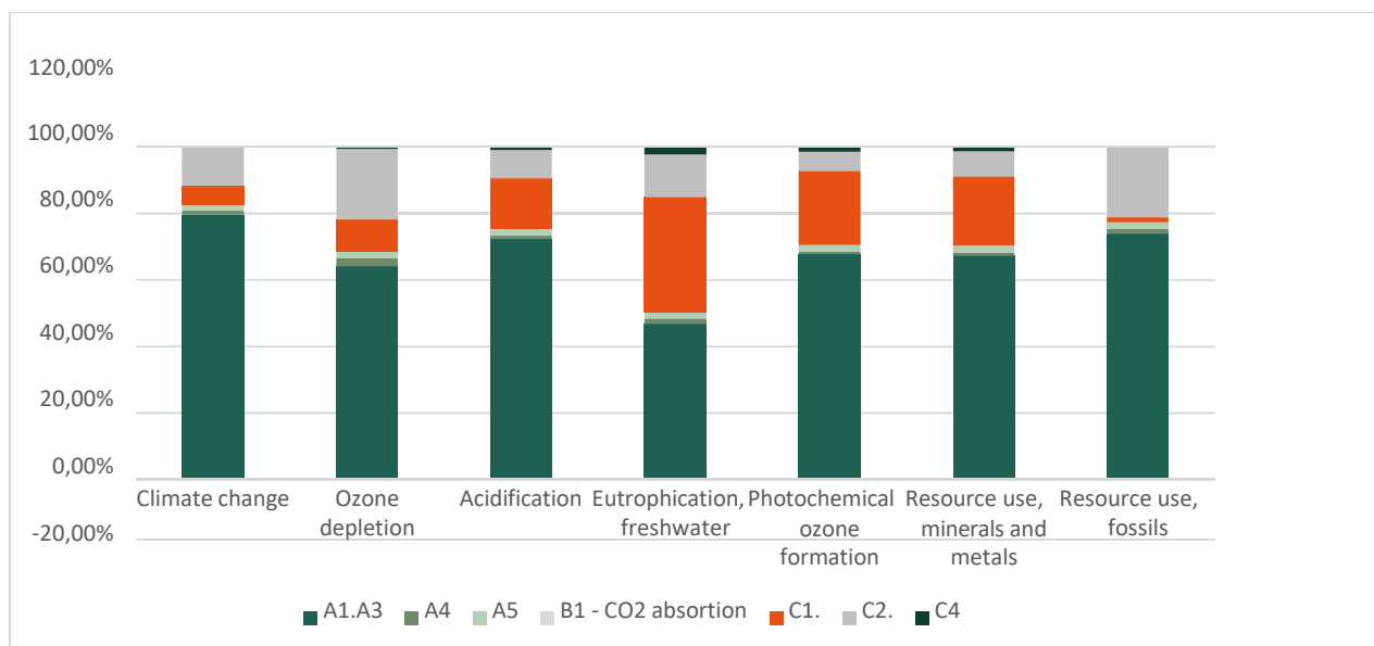
Figure. Potential impact on the environment of the life cycle of one m³ of ECOPact H30, H25, H25 AGILIA, H30 AGILIA, ARTEVIA HDOS 330 and HYDROMEDIA, in percentage.
